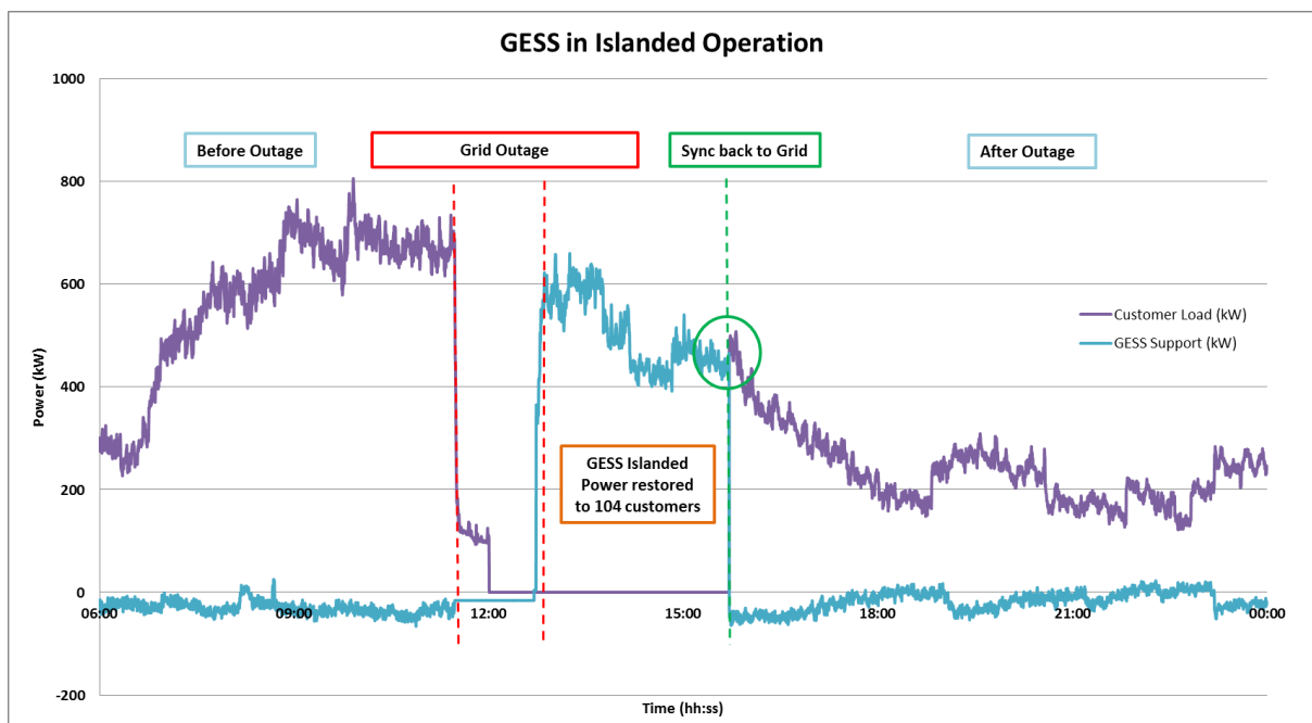
Fig 8: GESS supplying downstream customers during a network outage
