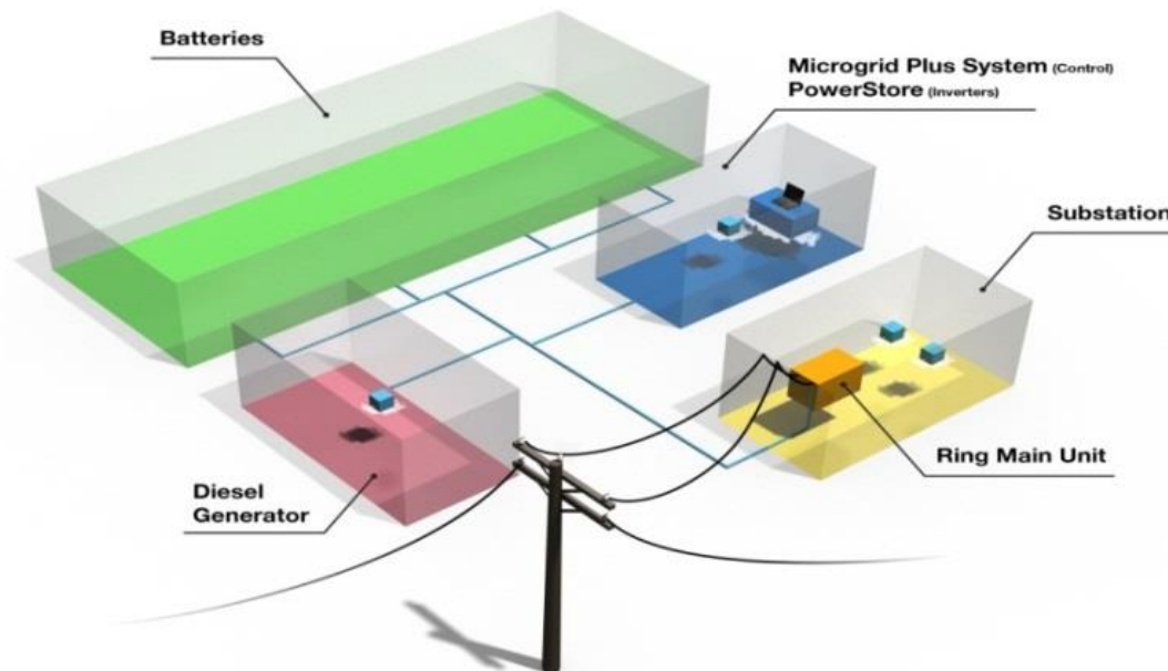
Fig 2: GESS system layout
