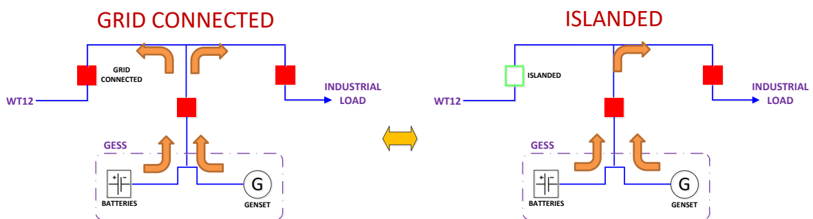
Fig 5: GESS network support modes for grid connected and islanded operation
