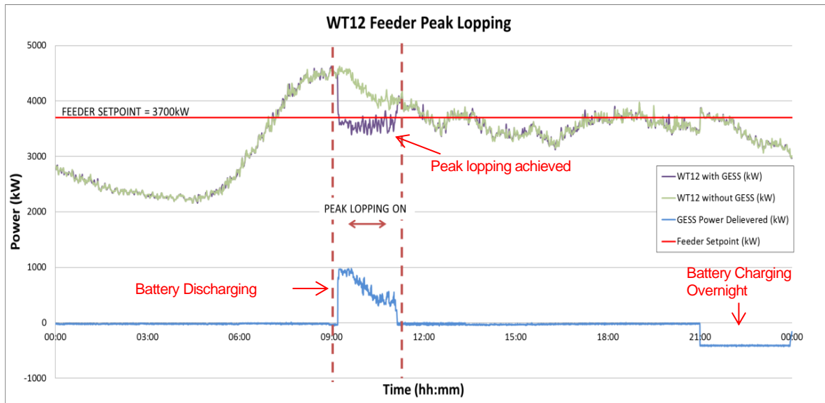
Fig 4: Example of feeder peak lopping on feeder WT12
